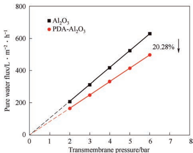
Fig. 3. Pure water flux of \text{Al}_2\text{O}_3 and \text{PDA-Al}_2\text{O}_3 tubular membranes.
