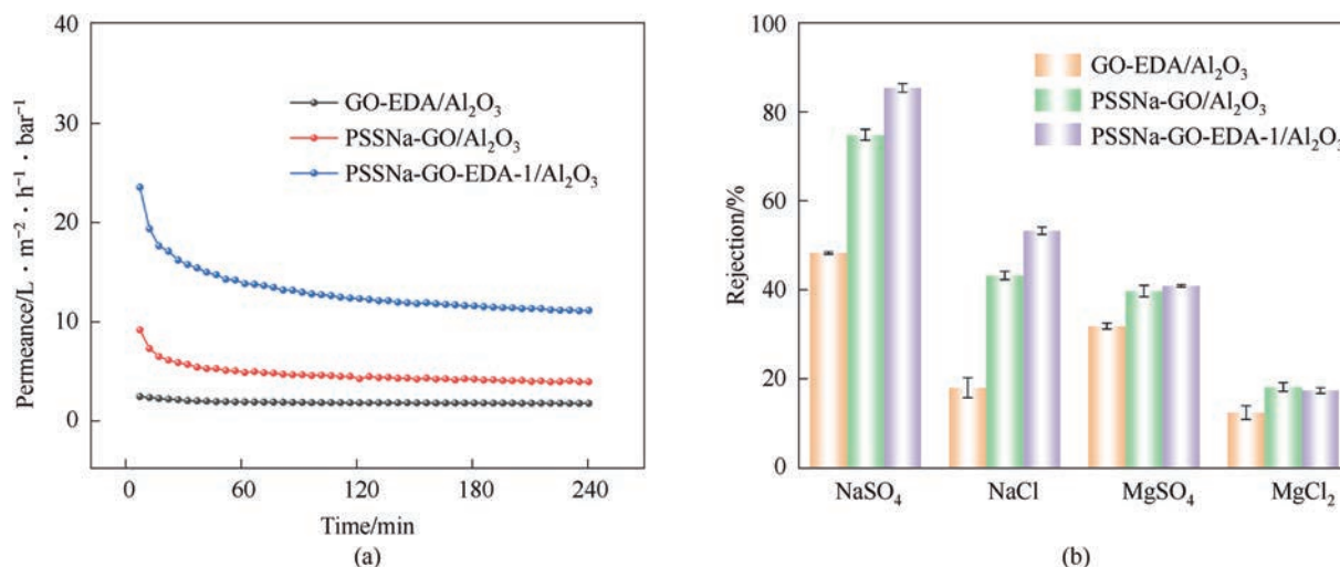
Fig. 13. Nanofiltration performance of GO-EDA, PSSNa-GO, PSSNa-GO-EDA-1 membrane: (a) pure water permeance (b) rejection performance for four salt solutions.
