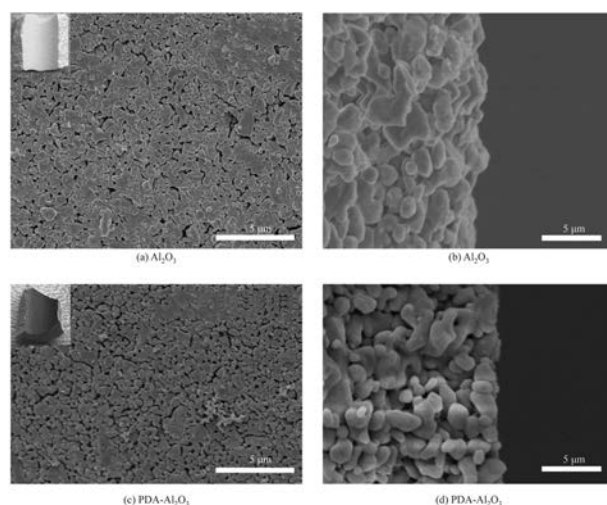
Fig. 2. SEM images of (a, c) surfaces, (b, d) cross-sections of the \text{Al}_2\text{O}_3 and PDA- \text{Al}_2\text{O}_3 membranes.
