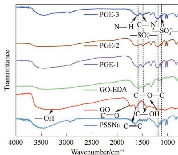
Fig. 5. FTIR spectra of PSSNa, GO, GE, and PGE membranes.
