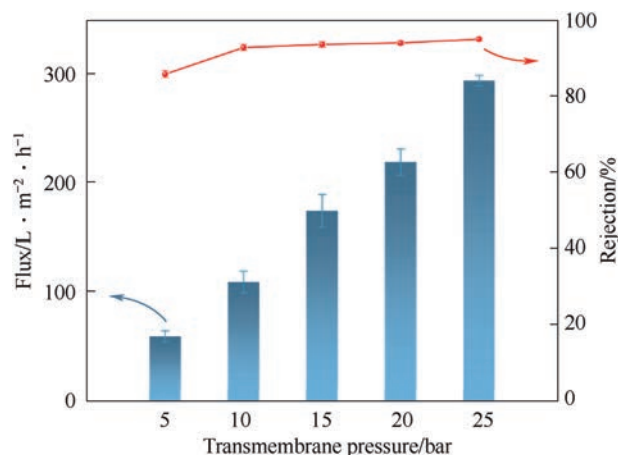
Fig. 15. Rejection of PGE-1 membrane towards 1 mmol·L -1 Na 2 SO 4 solution under 5, 10, 15, 20, 25 bar.
