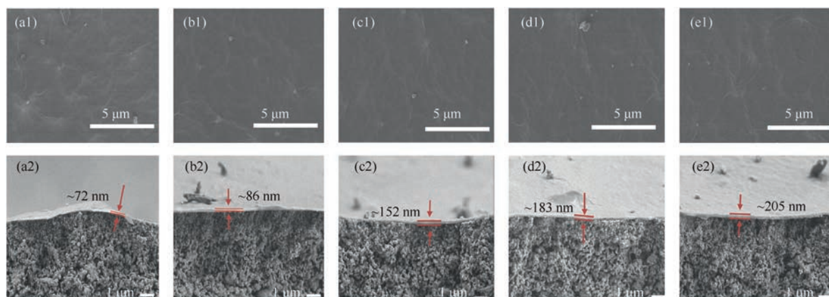
Fig. 7. SEM images of (a1) GO, (b1) GE, (c1) PGE-1, (d1) PGE-2, (e1) PGE-3 membrane surfaces and (a2) GO, (b2) GE, (c2) PGE-1, (d2) PGE-2, (e2) PGE-3 membrane cross-sections.
