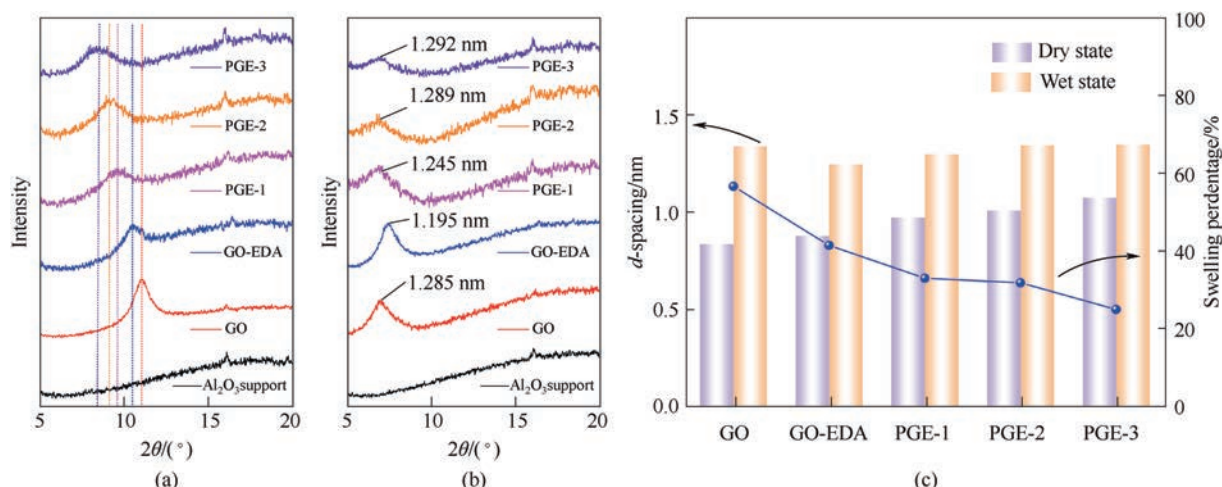
Fig. 9. XRD patterns of the GO-based membranes in the (a) dry and (b) wet states; (c) d-spacing and swelling percentage of GO-based membranes in dry and wet conditions.
