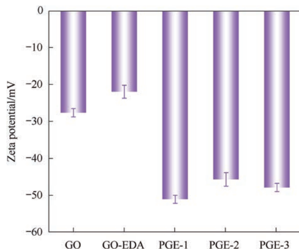
Fig. 4. Zeta potential of pristine GO, GE, PGE membrane-forming suspension.
