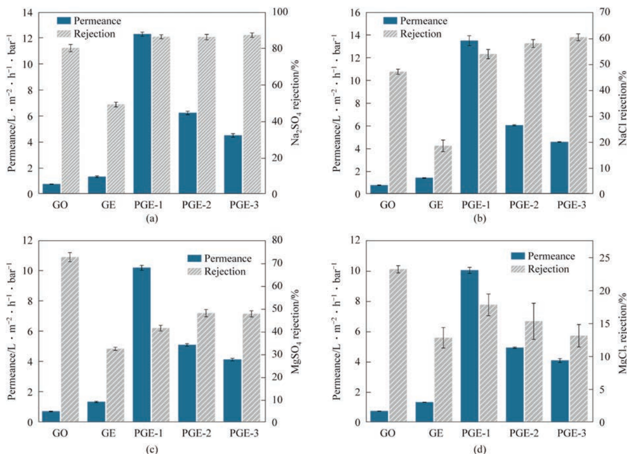
Fig. 11. Permeance and separation performance of GO and GE and PGE membranes towards four single-component salt solutions (a) \text{Na}_2\text{SO}_4 , (b) \text{NaCl} , (c) \text{MgSO}_4 , (d) \text{MgCl}_2 .
