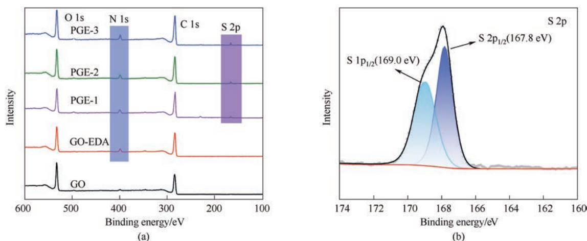
Fig. 6. (a) XPS full-scan spectra of GO, GE, and PGE membranes; (b) S 2p spectra of PGE-1 membrane.
